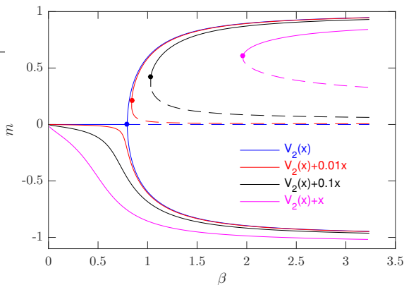
Figure: Bifurcation diagrams of m as a function of \beta for tilted bistable potentials with a_0 = 0.25 , and \kappa = 0, 0.01, 0.1, 1 (see legend). Here, we used \theta = 2.5 . The symmetric pitchfork bifurcation is broken at any \kappa > 0 . Note that the locus of the critical points forms a distinct critical line.
